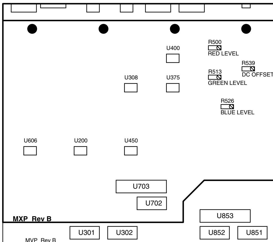
FIGURE 1 - MVP-24X COMPONENT LOCATIONS.
